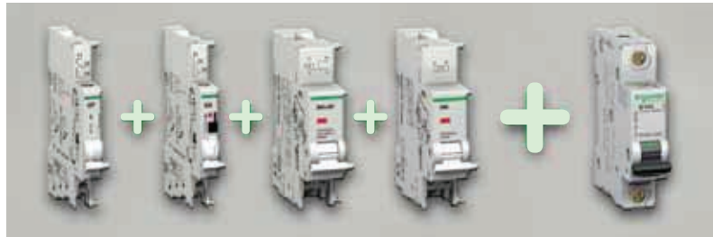
SD Alarm Switch OF Auxiliary Switch MX Shunt Trip + Aux Switch MN Undervoltage Release C60
