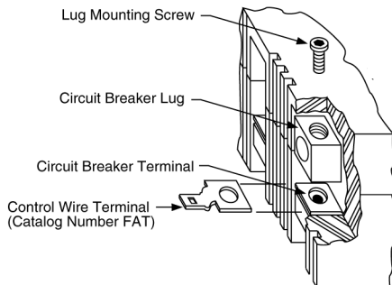
Installing AL250KAT
