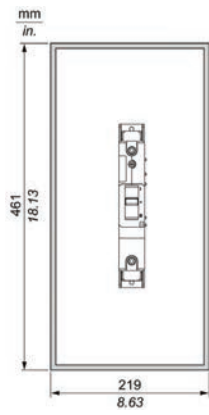
1P Front View
