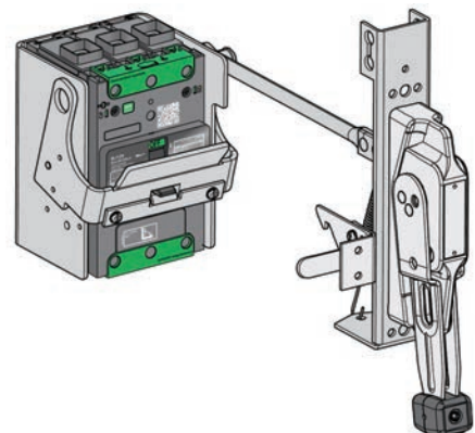
9422 Operating Mechanism with Flange-Mounted Handle
