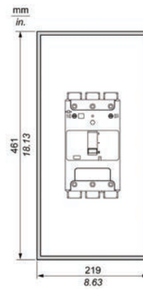
3P/4P Front View
