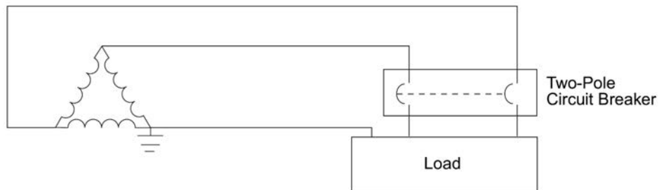
Three-Phase 240 Vac Corner-Grounded Delta System.
