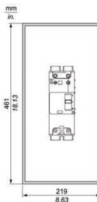
2P Front View
